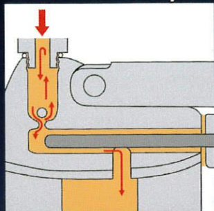
without TWIN-LOCK-System
