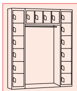
Archway Locker - H.1800 W.1800 D.450
