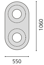
Plan view
