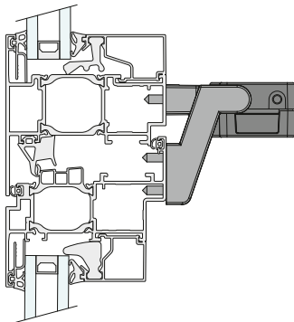
Universal bracket sets, outward opening
