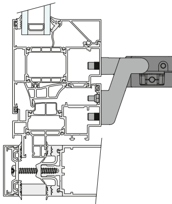
Façade windows, outward opening
