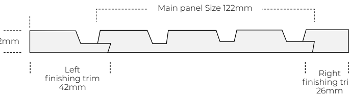
Panel and finishing trim dimensions
