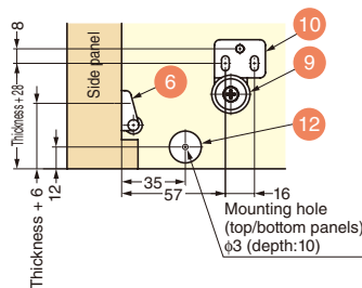
Cross section b: For roller bracket mounting
