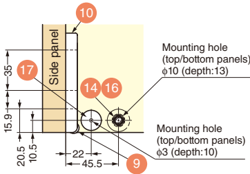
Cross section b: For mounting with female screw
