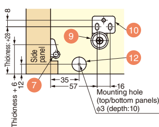
Arrow view b: For roller bracket mounting
