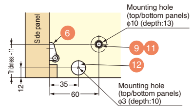
Cross section b: For mounting with female screw
