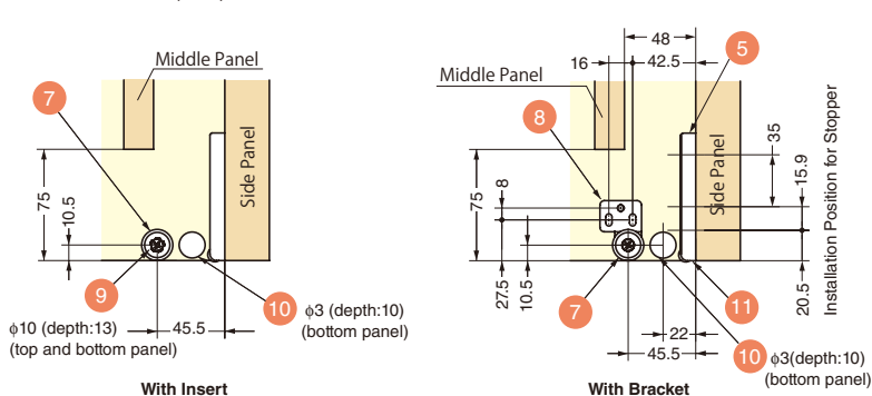
Cross section B (P.29)
