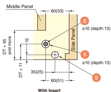
Cross section B (P.12)
