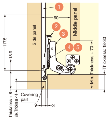
Cross section a: Slide/hinge mounting
