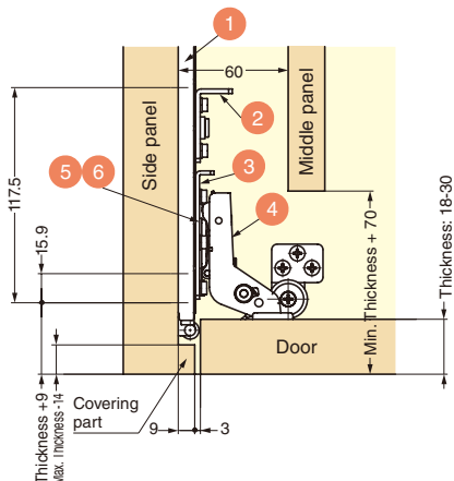
Cross section a: Slide/hinge mounting
