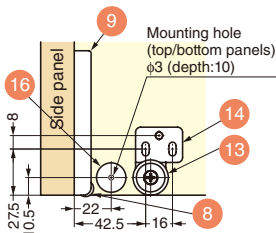
Cross section b: For roller bracket mounting
