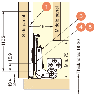
Cross section a: Slide/hinge mounting
