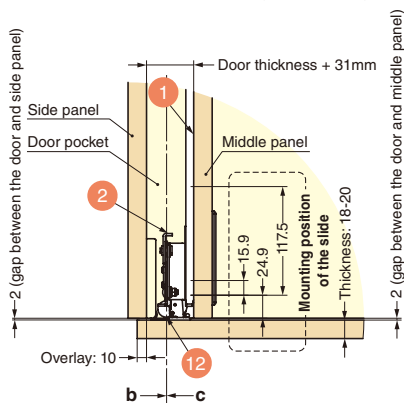
Cross section a: Slide/hinge mounting
