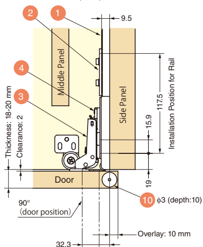
Cross section A (P.29)
