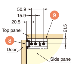
Cross section c
