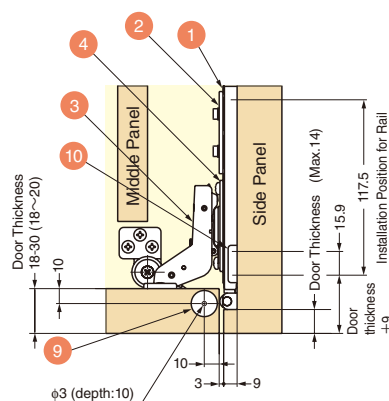
Cross section A (P.12)
