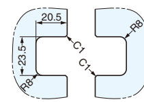
Transparent bumper (included)
