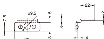
Strike for inset door (included)
