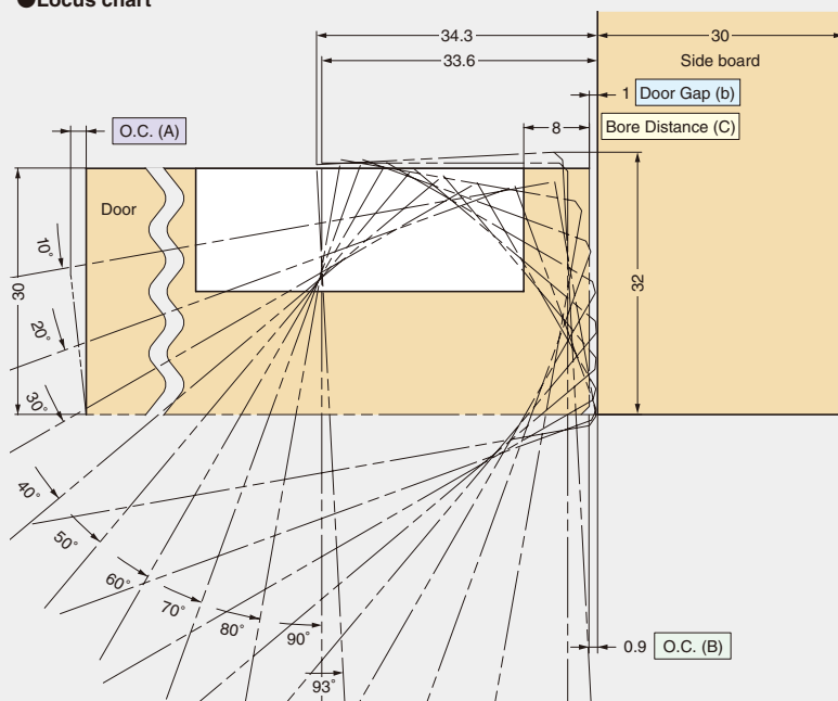
Drawing above is J95-C24/OT Bore Distance 8 mm, Door Thickness 30 mm, Side Board Thickness 30 mm.
