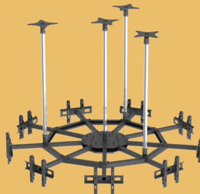
Example Heavy Duty Nonagon Spider Gantry - Supported 9x 43" Sony Screens -
