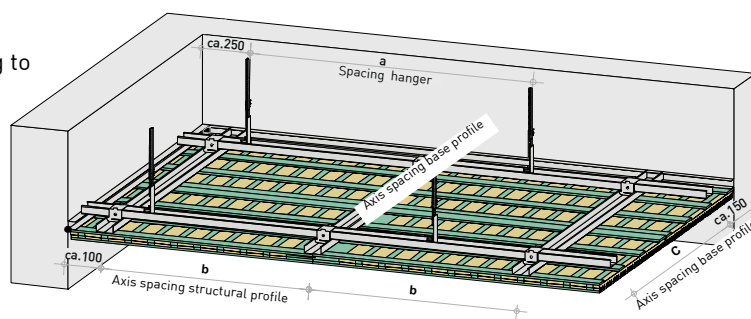
Continuous UD-profile for wall area connection
