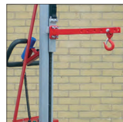
Jib and Hook - EP07 500mm long Capacity: 150kg
