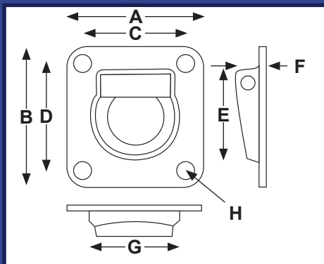
CAT310 Single Recessed Lashing Ring - Rope Fitting No.310
