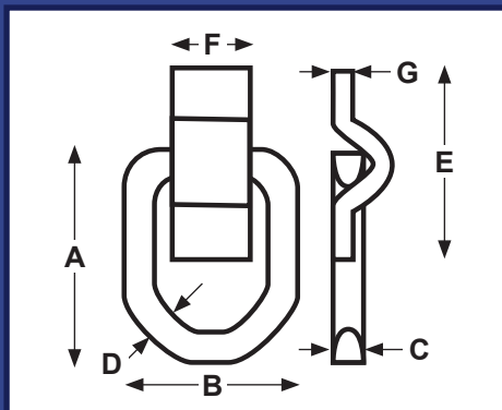
1060/001 Ferry Lashing Ring
