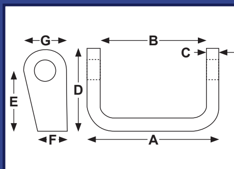
RG999/C - G Universal Bolt on Hinge Bracket
