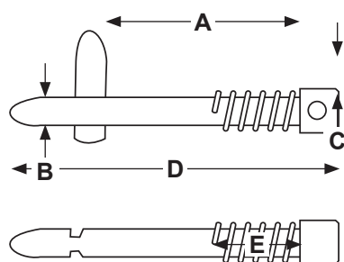
IR206 Spring Loaded Sword Pin
