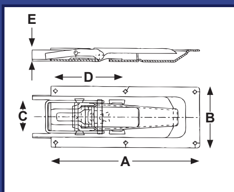
IR694B Overcentre Spring Loaded Toggle Fastener
