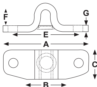
RG150 Mounting Bracket
