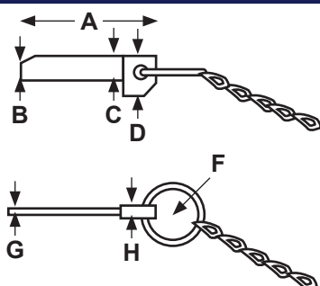
IR10A Flat Drop Forged Cotter
