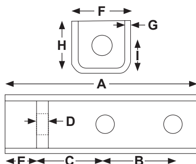
RG137/5 Scania Lower Mounting Bracket
