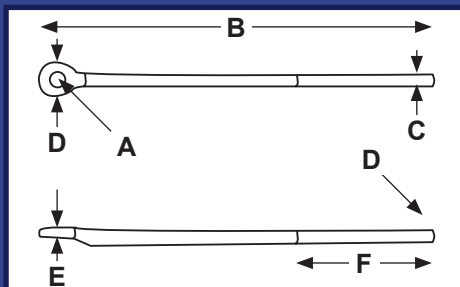
IR754/5 Tie Bar - 16mm and 12mm
