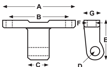
IR209/300A Jagalok Hinge Housing
