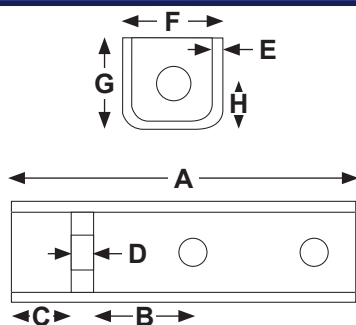
RG137 Scania Lower Chassis Bracket
