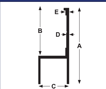
Dropside End Cap
