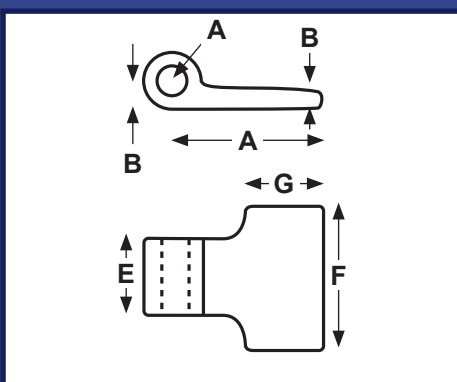
IR119 Drop Forged Hinge - Weld On
