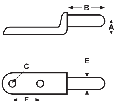
IR22 Hinge Hooks
