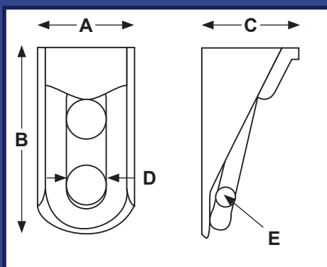
CAT250 Floor Lashing Ring
