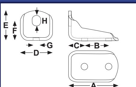
RG113R Mounting Bracket
