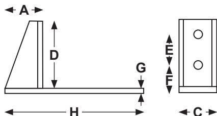
IR706B Fabricated Pedestal Mounting Bracket
