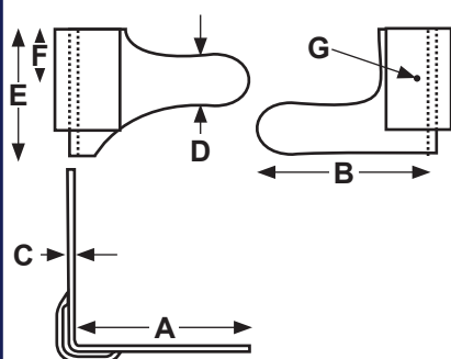
IR306L/R Socket for Corner Pillar
