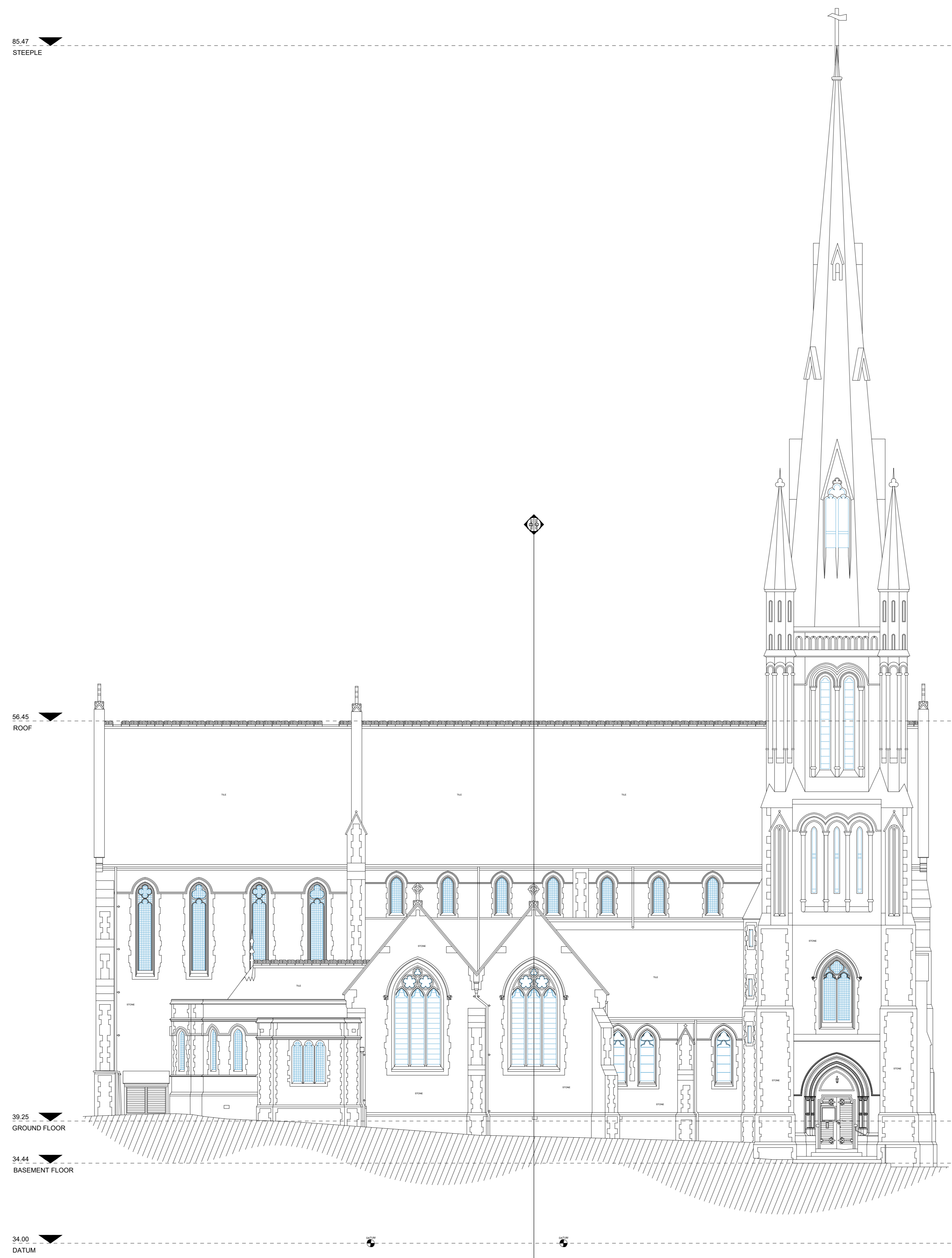
NORTH WEST ELEV
