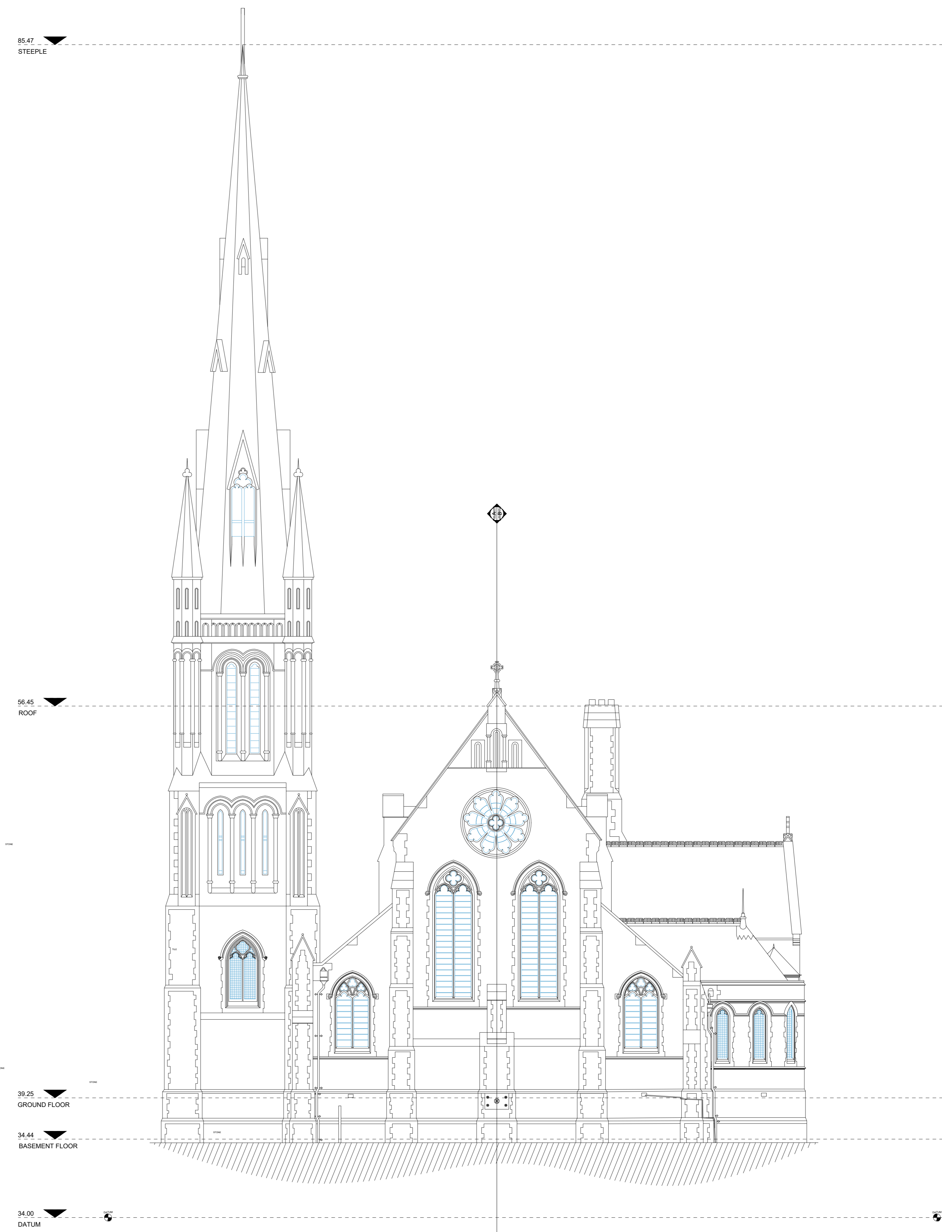
SOUTH WEST ELEV
