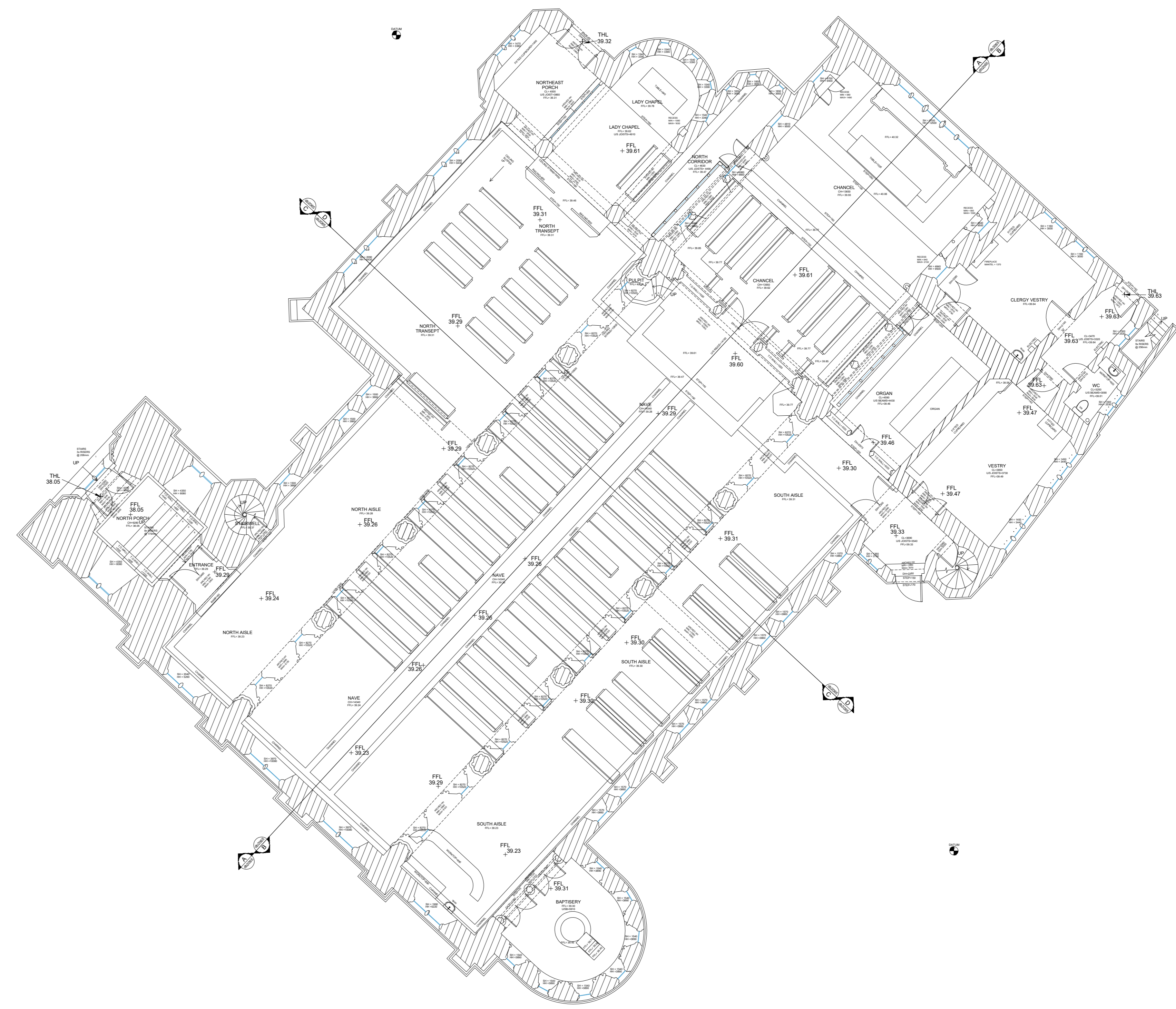
GROUND FLOOR
