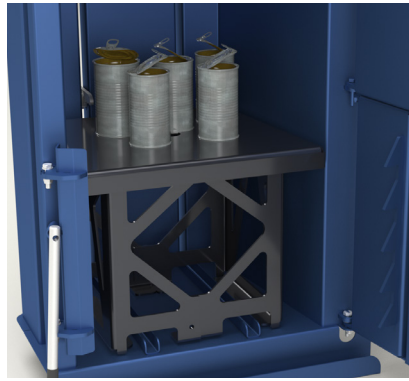
Can crusher insert Internal insert for crushing cans up to 30 litres and similar rigid containers.
