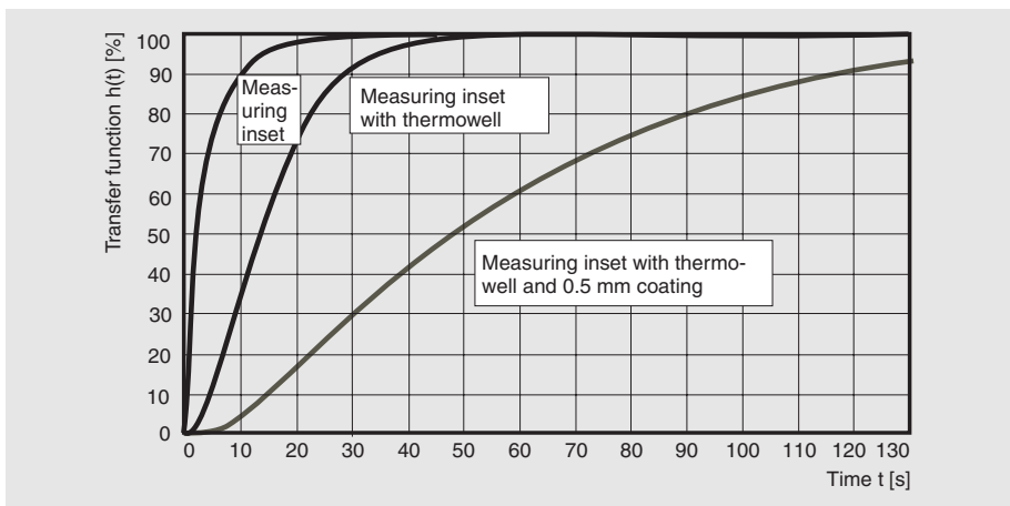
Fig. 3-55: Transfer function for resistance thermometers of different designs in water v_W = 0.4\text{ m/s} (16 ft./s), T_W = 25\text{ }^{\circ}\text{C} (77 ^{\circ}\text{F} )
