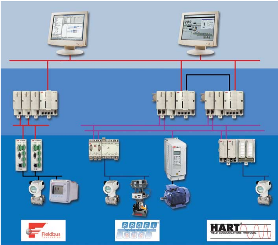
Fig. 5-25: Decentralized redundancy capable fieldbus interface components (with integrated HART or fieldbus communication)
