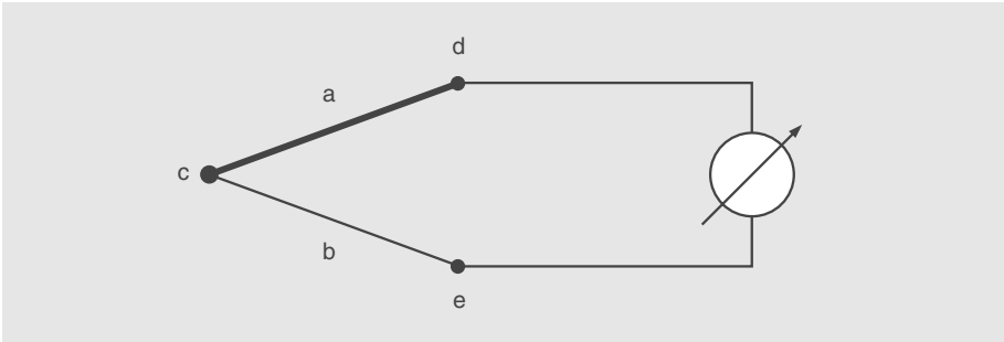
Fig. 2-4: Thermal circuit: c = Metering point; a, b = Thermal legs; d, e = Reference junction
