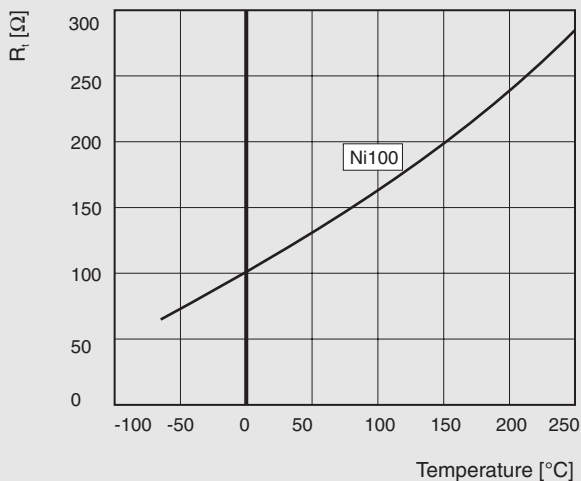
Fig. 3-6: Relationship of the resistance R_t to the temperature for Ni100
