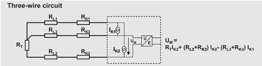
Fig. 5-5: Circuit diagram of a three-wire circuit
