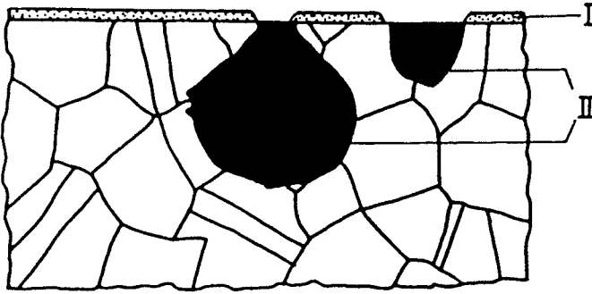
Fig. 3-30: Pitting corrosion schematically
