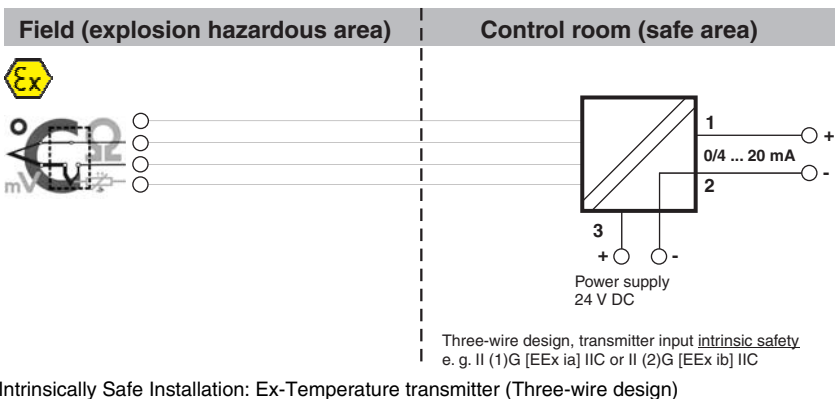
Fig. 5-20: Installation of temperature transmitters in explosion hazardous areas
