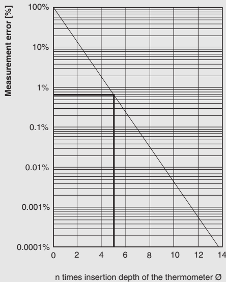
Fig. 6-2: Dependence of the thermal loss errors to the ratio of the insertion depth to the diameter of a temperature sensor for liquids
