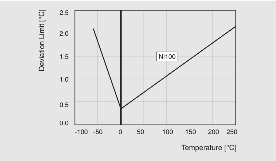
Fig. 3-7: Maximum deviation limit in °C for Ni100
