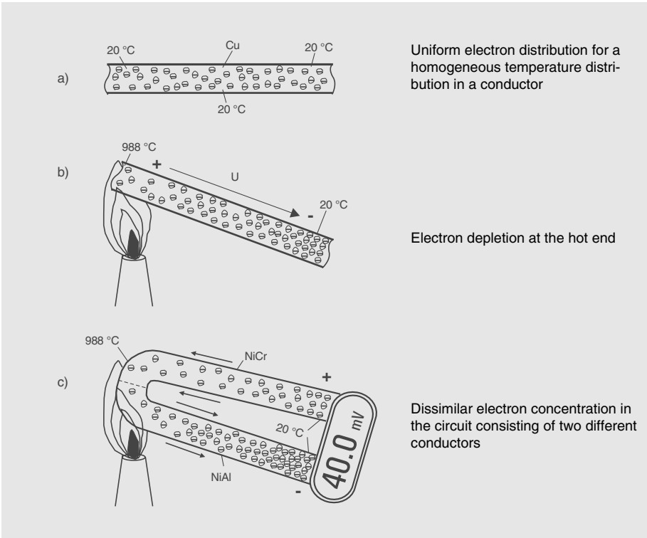
Fig. 2-2: Generation of a thermal voltage
