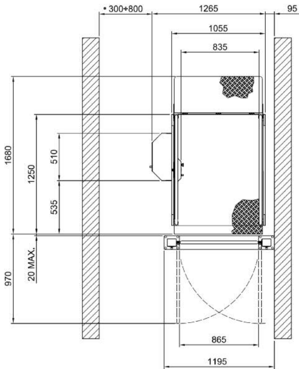
"STANDARD" VERSION, RH - STRAIGHT EXIT
