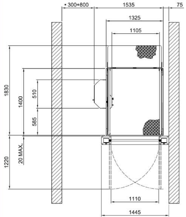
"LARGE" VERSION, RH - STRAIGHT EXIT
