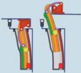
Gear hinge with moving pivot point for high load
