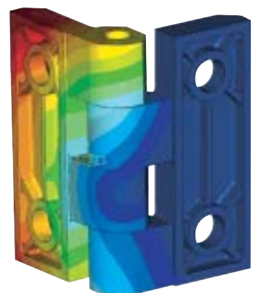
Using FEM to help optimize product design
