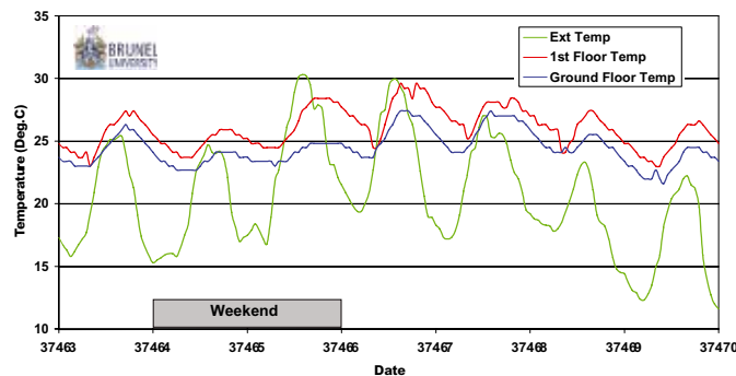
Ground floor and first floor temperature profiles in relation to external air temperature from 26/07/02 to 02/08/02 at the Tonbridge and Malling council offices, Kings Hill (External temperatures provided by the Met office)
