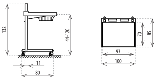
BSR119: Free-standing changing table with wheels
