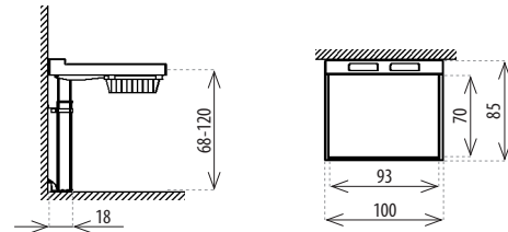
BSR121: Wall-mounted changing table, single column
