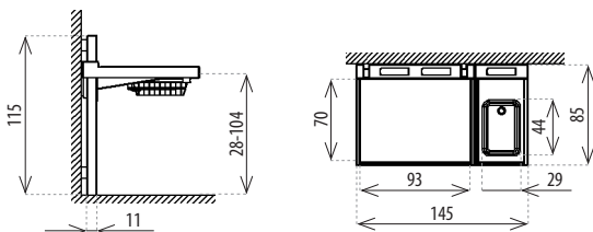
BSR107: Wall-mounted changing table with sink
