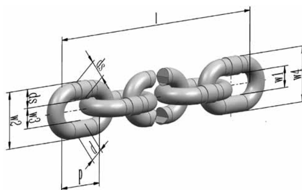
Chain dimensions round steel chain
