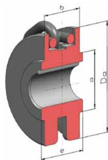
Type B: with shoulders
