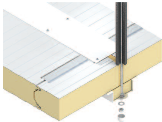
ColdZone Ceiling Support
