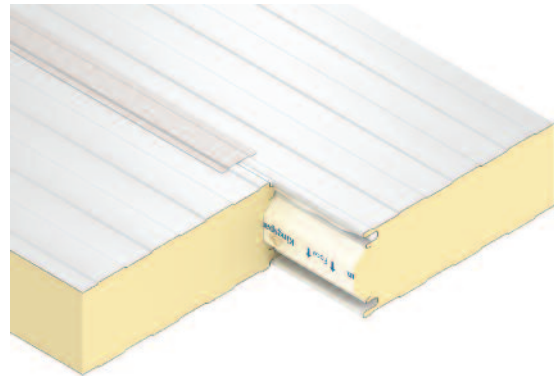
ColdZone Ceiling Panel Joint
