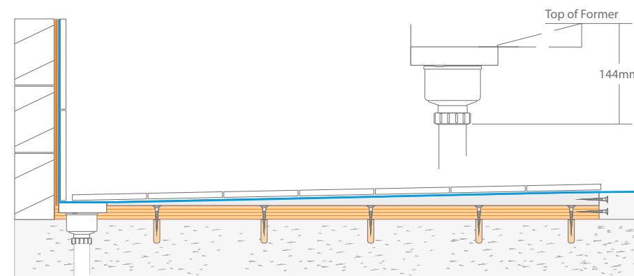
OTL INFINITY I-LINE LINEAR CHANNEL ON A CONCRETE SUB-FLOOR
