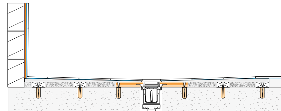
OTL SUPERSLIM CHANNEL ON A CONCRETE FLOOR
