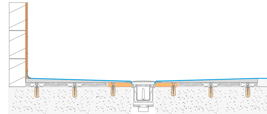
OTL RESIN FORMERS ON A CONCRETE FLOOR
