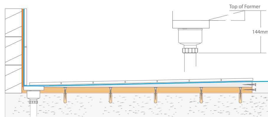
OTL INFINITY I-LINE LINEAR CHANNEL ON A CONCRETE SUB-FLOOR
