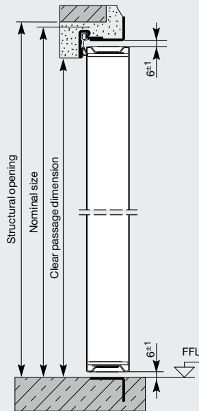
Shown without threshold profile
