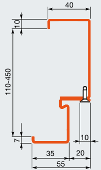
Standard special corner frame, on request with counter frame
