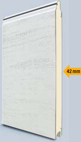
LPU 40 Double-skinned door leaf 42 mm thick
