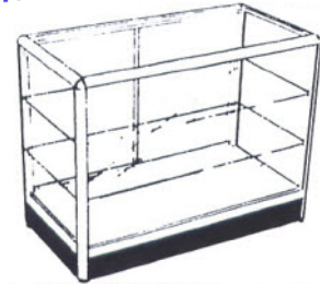
A. COUNTER SHOWCASE £565.00 With glass shelves. 1000W x 500D x 900H
