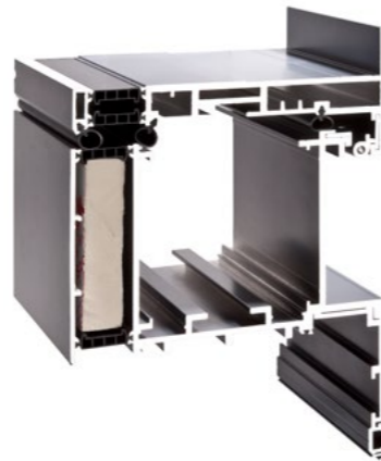
Thermally broken aluminium frame with 39mm polyamide thermal breaks and closed cell PIR insulation.
