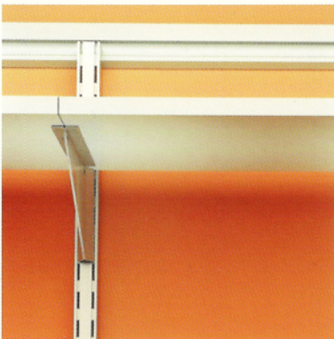
Pass-over bracket double flange
