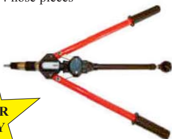
Insert Tool For easy setting of rivet nuts up to M10
