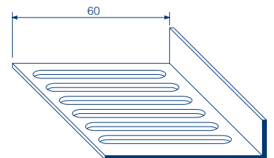
C065 (25 mm type) 60 x 15 mm Angle ventilator
