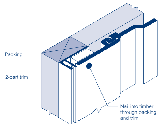
Fig.33 Finishing with a cut plank
