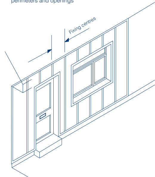
Fig. 3 Fix intermediate vertical battens at appropriate centres
