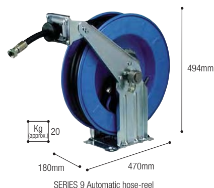
SERIES 9 Automatic hose-reel
