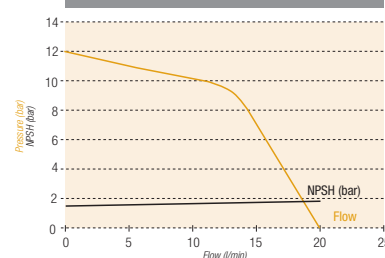
Flow curves
