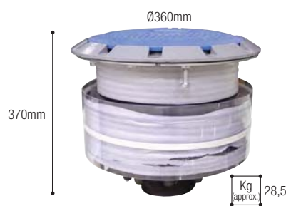
4" manhole container with fibre cover
