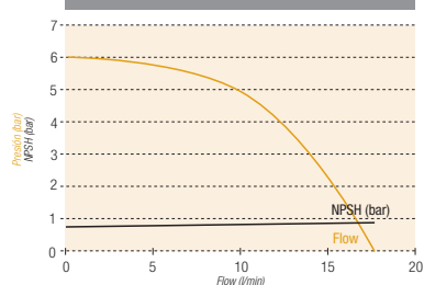
Flow curves
