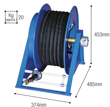
SERIES 5 Automatic hose-reel
