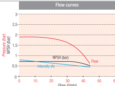
AG-500 230VAC
