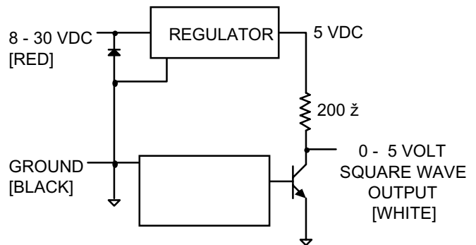
ELECTRONIC FUNCTIONAL DIAGRAM
