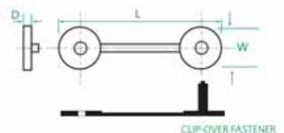
CLIP-OVER FASTENER
