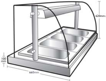
Heated Displays - Bains Marie Full height glass screen with side cheeks and flat GN collar.
