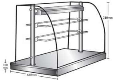
Ambient Displays - Two Tier Full height glass screen and side cheeks.
