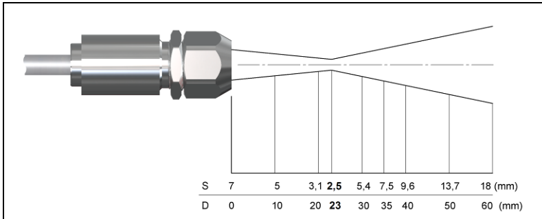
LT02 with CF lens (2,5 mm@ 23 mm)
