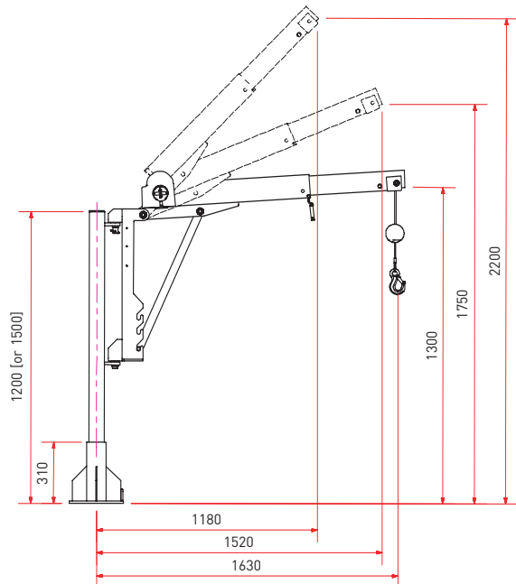
ML500 pickup, dropside & flatbed type
