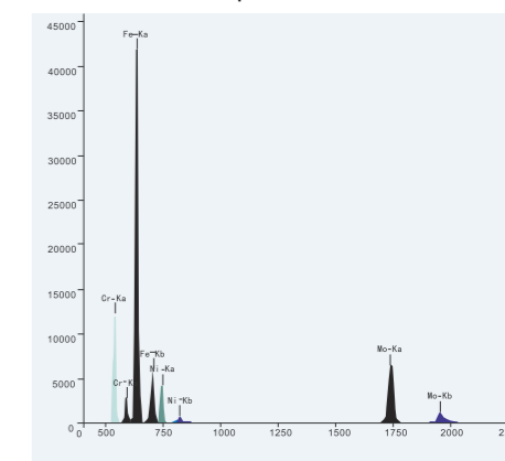
Spectrum of 316 Stainless Steel
