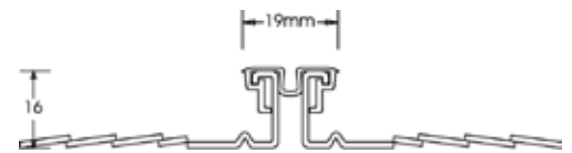
MBG3019 / MBS3019 19mm Movement Bead
