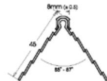
1046 45mm c/w PVCu Nose Angle Bead
