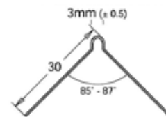
LCG135 25mm Wing 135° Angle Thin Coat Bead
