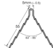
LWG64 / LWS64 64mm Long Wing Angle Bead
