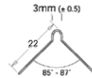
LCG 25mm Long Wing Thin Coat Bead
