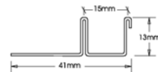
1314 Feature Bead with 10mm Gap
