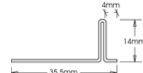
1304 Feature Bead with 10mm Gap
