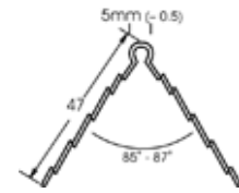
LWG53 / LWS53 53mm Long Wing Angle Bead
