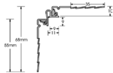
IMG3013 / IMS3013 13mm Internal Corner Movement Bead
