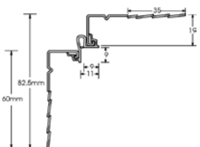
IMG3019 / IMS3019 19mm Internal Corner Movement Bead
