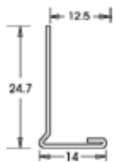
EBG3010 / EBS3010 9.5mm Edging Bead
