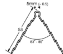
MAX55 55mm Long Wing Angle Bead
