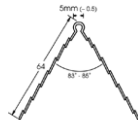
1046 45mm c/w PVCu Nose Angle Bead
