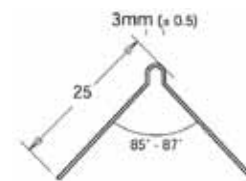
LCG(30) 30mm Thin Coat Bead
