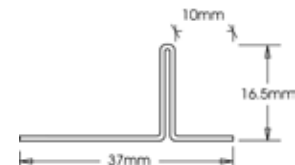
1377 Feature Bead with 5mm Gap
