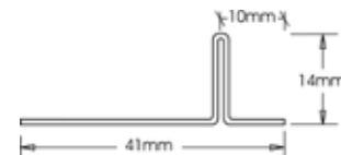
1371 Feature Bead with 4mm Gap
