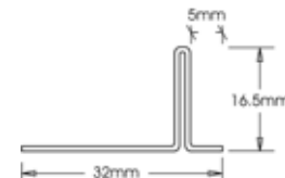
1377 Feature Bead with 5mm Gap
