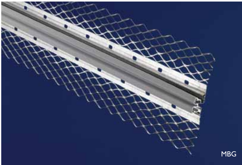
MBG3010 / MBS3010 10mm Movement Bead
