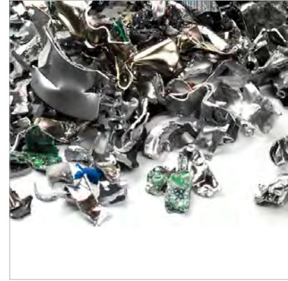
Particles of shredded hard drives Cutting size: 11,5 x 26 mm (<299 mm 2 ). Security level: H-5
