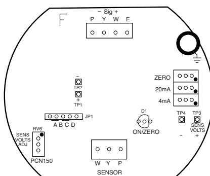
EEExd SENSOR BOARD
