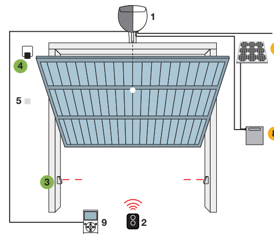
Projecting up-and-over door
