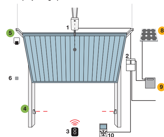
Non-projecting up-and-over door
