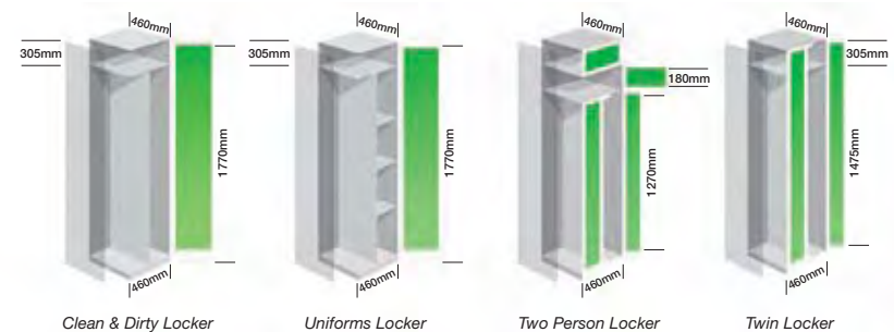
Clean & Dirty Locker Uniforms Locker Two Person Locker Twin Locker
