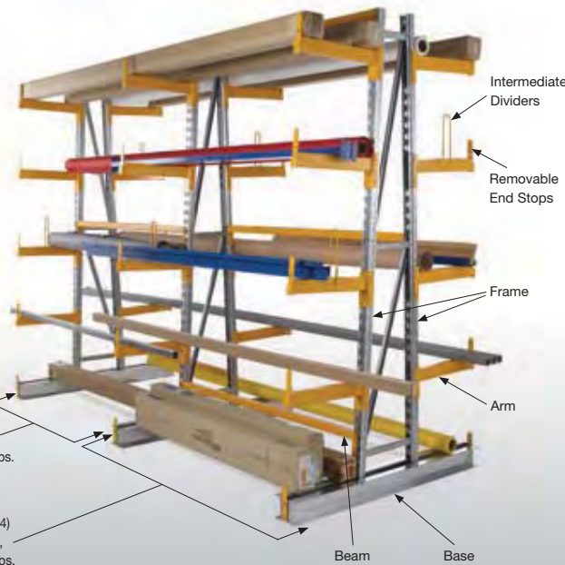
Single Sided Starter Bay Double Sided Starter Bay
