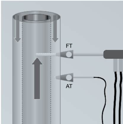
Fig. 12: Measurements on balanced flue systems
