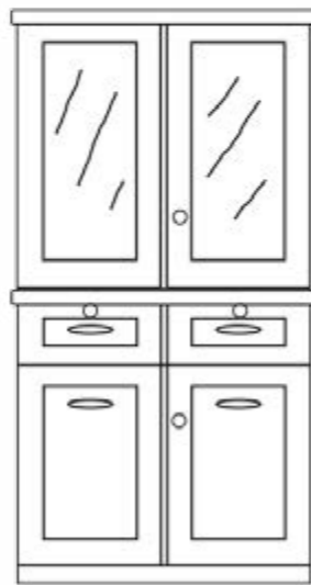
Sideboard with Dressing Top H1890 W1000 D510
