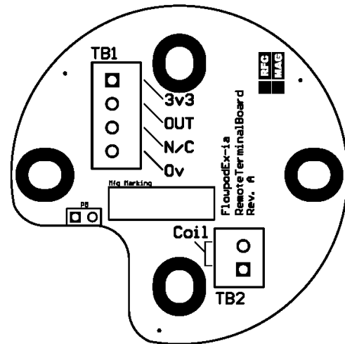
Remote terminals (RF/Mag Coils) Rev.A
