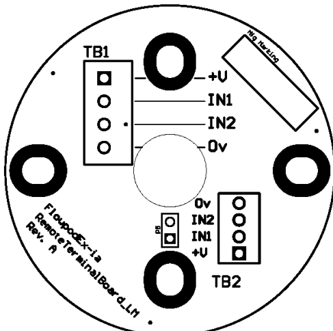
Remote terminals LM (Pulse signals) Rev.A
