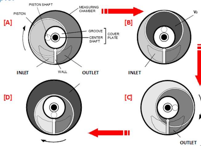
Figure 1 Measurement Principle
