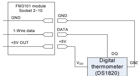
Figure 5. Digital thermometer DS1820 connection scheme
