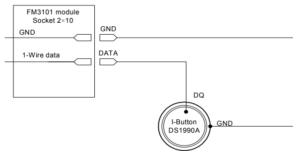
Figure 6. Digital key “I-Button” DS1990A connection scheme
