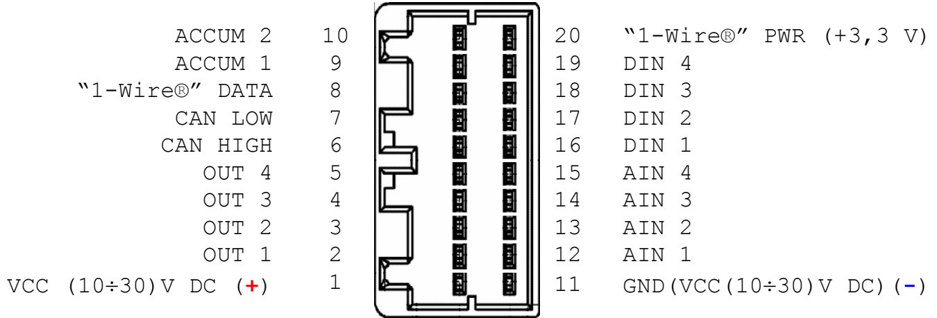
Figure 2. 2x10 socket pinout
