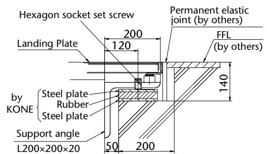
Escalator Mounting Detail X / Y
