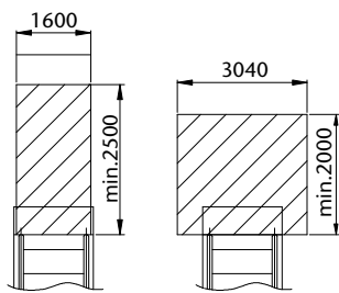
Passenger Circulation Area Requirements
