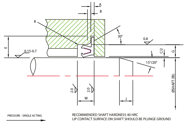
F700 Rotary Shaft Seal
