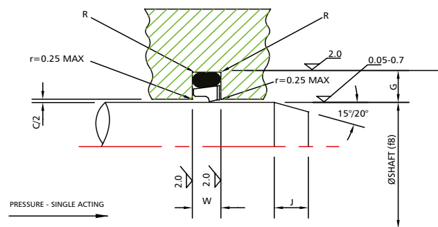
F300R Rod Seal
