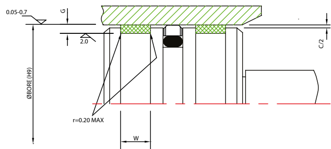
F800R Internal Acting Bearing Strip
