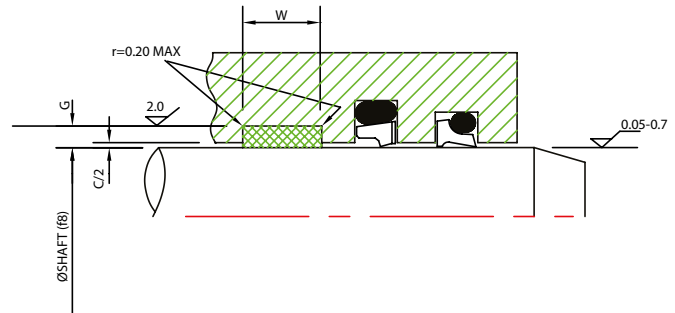
F800R Internal Acting Bearing Strip
