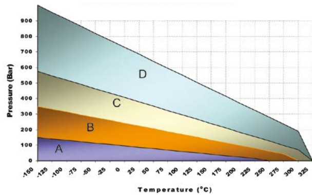
Figure 1, Temperature/Pressure Chart
