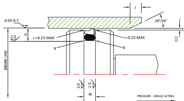
F300B Piston Seal
